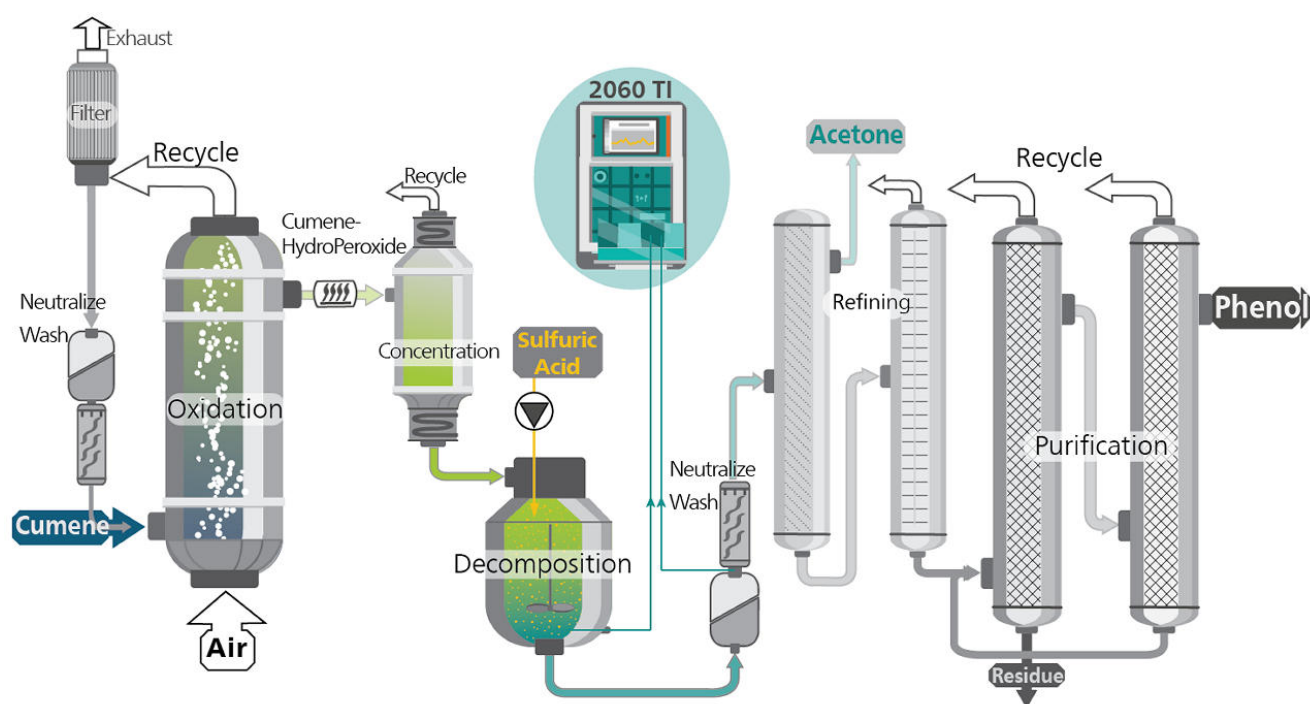
Figure 1. Simplified schematic showing how phenol is produced from cumene.
