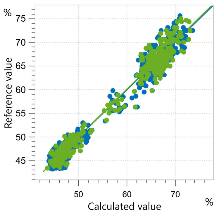
Figure 3. Correlation diagram and the respective FOMs for the prediction of protein content in fish meal using an OMNIS NIR Analyzer Solid. The calibration dataset is shown in blue, and the external validation dataset is in green.
