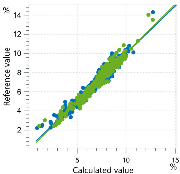
Figure 5. Correlation diagram and the respective FOMs for the prediction of moisture content in fish meal using an OMNIS NIR Analyzer Solid. The calibration dataset is shown in blue, and the external validation dataset is in green.
