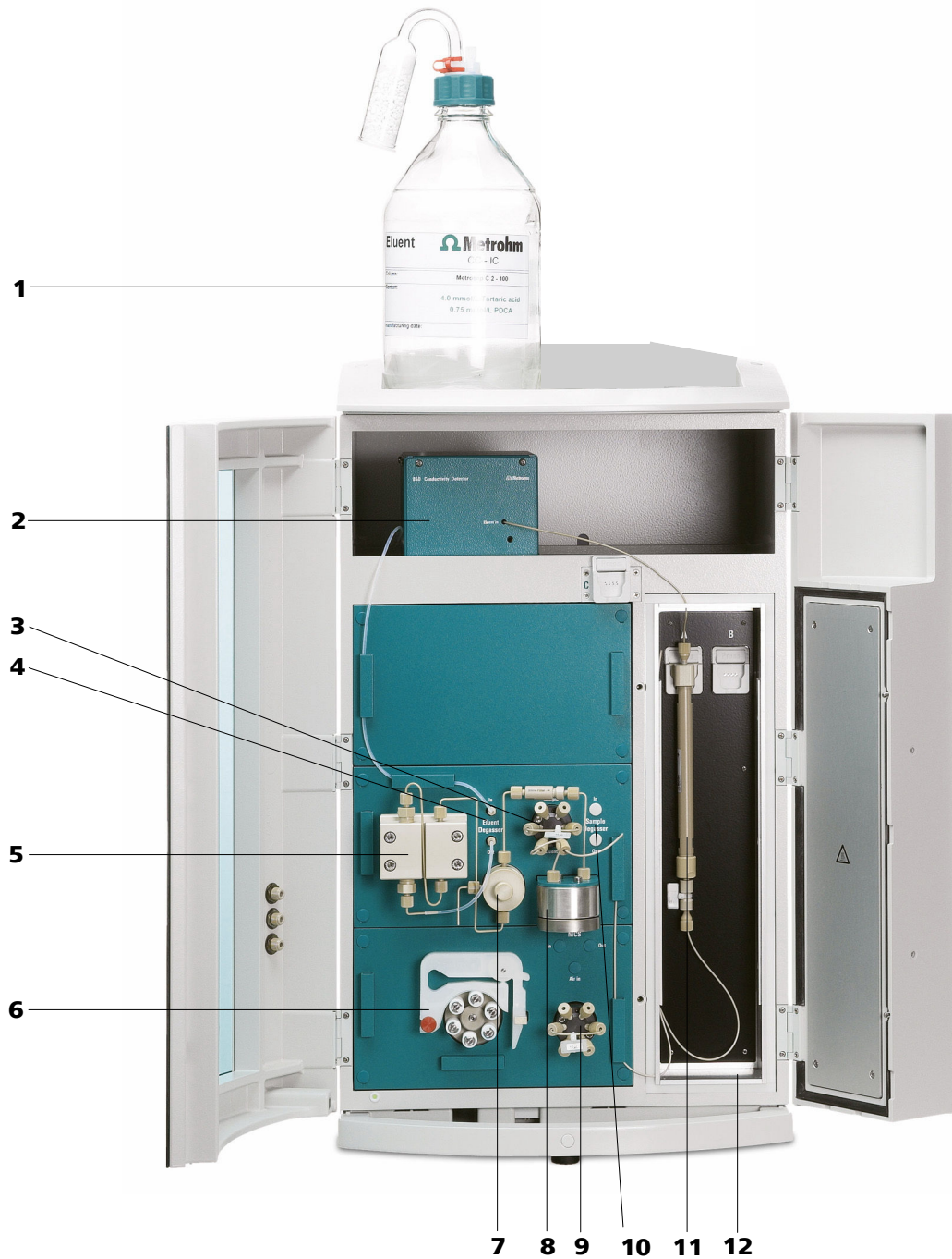
Figure 1 Front view of the instrument
