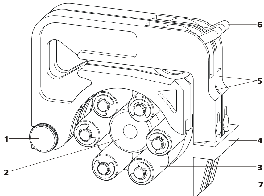
Figure 23 Peristaltic pump
