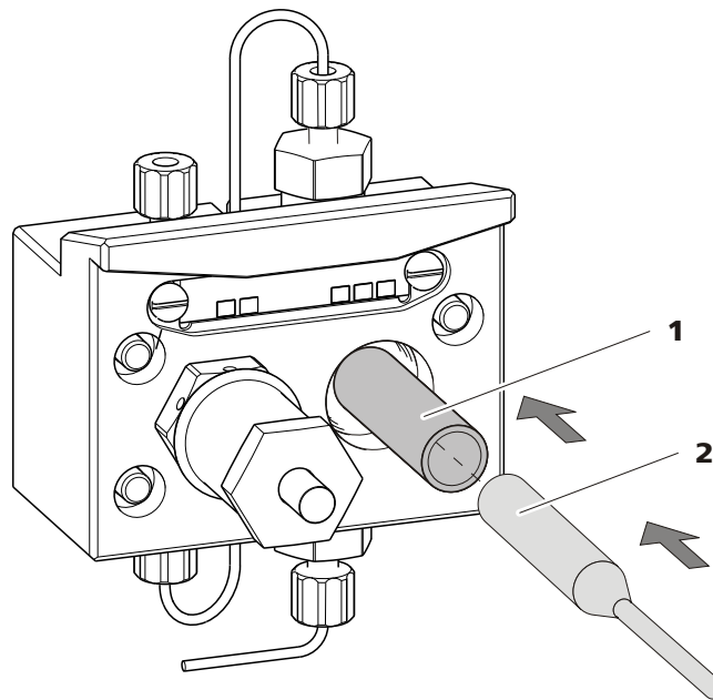
Figure 38 Inserting the piston seal into the pump head
